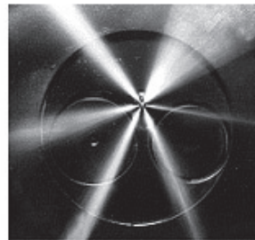
Deposit restricted diesel injector spray pattern
